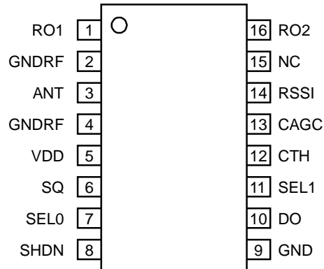
16-Pin QSOP (QS) (Top View)
