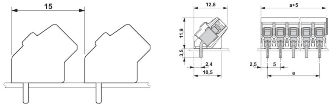
Dimensioned drawing
