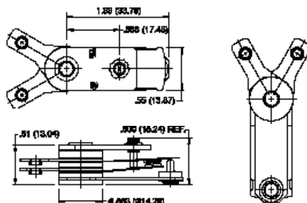
TOR Model - Fixed Thermostat
