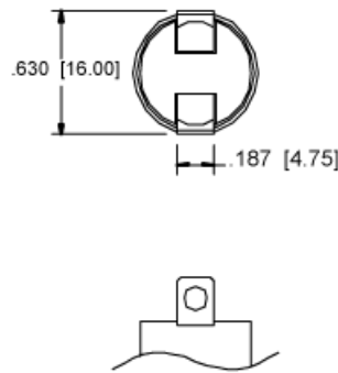
Code SV Solder • Vertical
