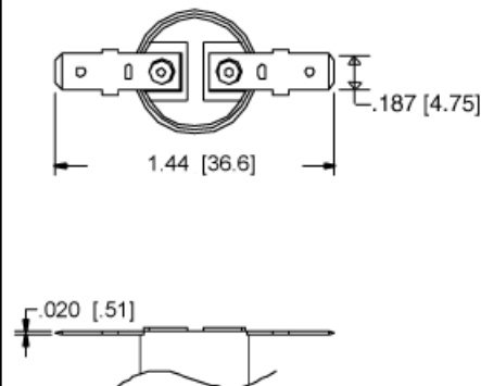
Code TH .187 Quick Connects • Horizontal
