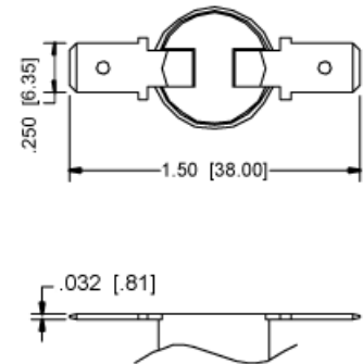
Code BH .250 Quick Connects • Horizontal
