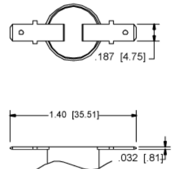
Code T3H .187 Quick Connects • Horizontal
