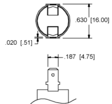
Code TV .187 Quick Connects • Vertical
