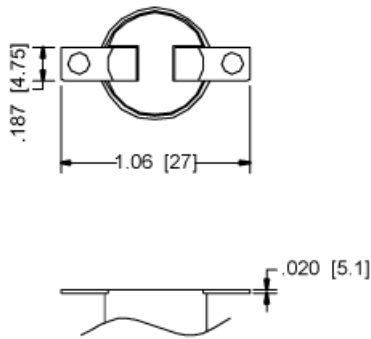
Code SH Solder • Horizontal
