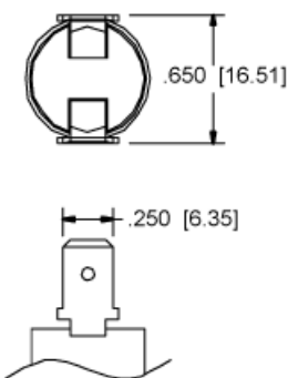
Code BV .250 Quick Connects • Vertical
