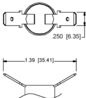
Code BQF .250 Quick Connects @ 30°
