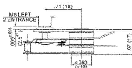
TL 02 Model Fixed Thermostat
