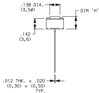
PTS645SL43TR SPST
