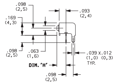
PTS635VL31 SPST
