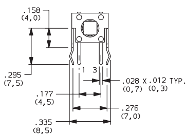
PTS645VJL61 SPST
