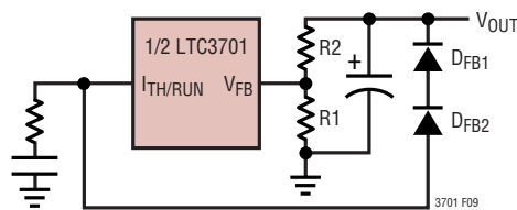
Figure 9. Foldback Current Limiting
