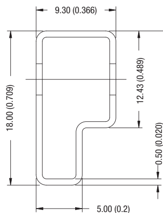
4 Pin SIP Tube
