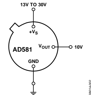
Figure 2. Pin Configuration (Bottom View)
