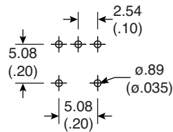
P.C. Mounting
