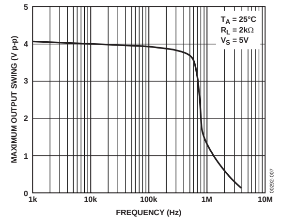
Figure 7. OP183 Maximum Output Swing vs. Frequency @ 5 V
