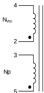
Figure 38. Inductor Schematic Diagram
