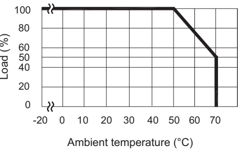
Output power vs. Ambient temperature
