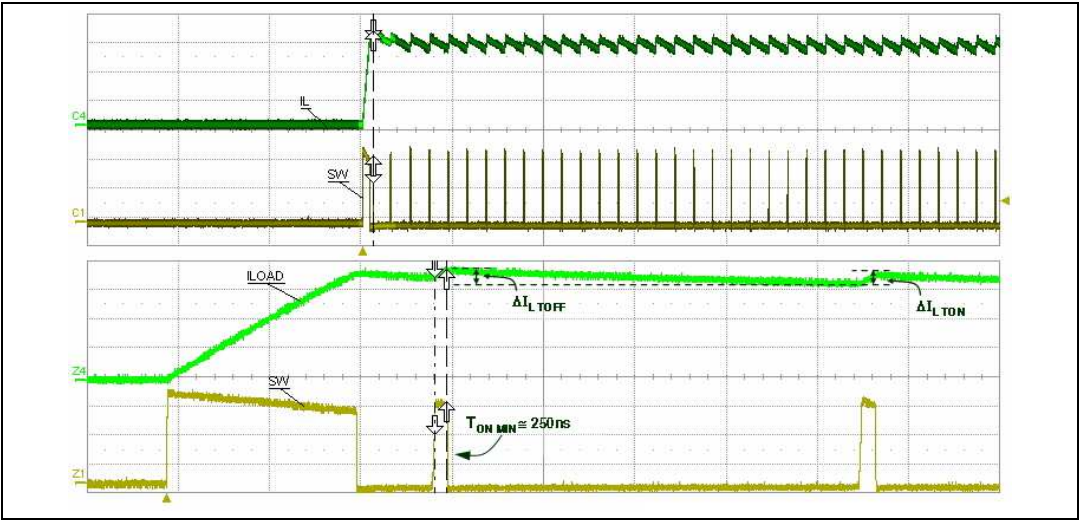
Figure 19. Short-circuit current V_{IN} = 12\text{ V}
