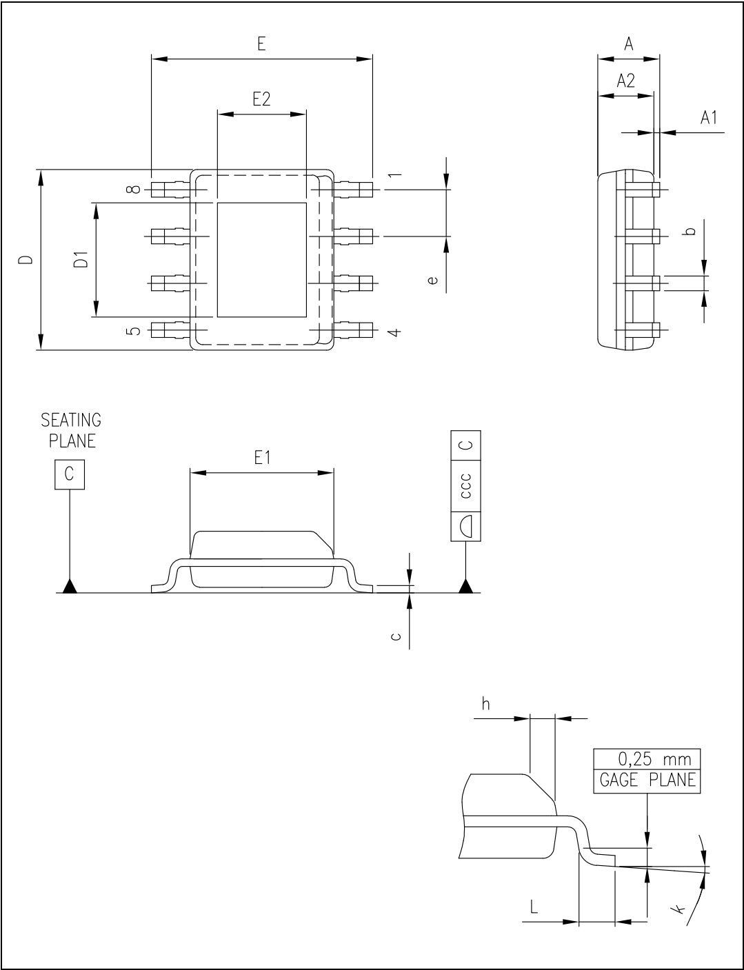
Figure 42. Package dimensions
