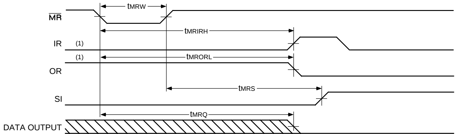
Figure 8. Master Reset Timing
