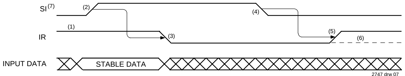
Figure 2. Input Timing
