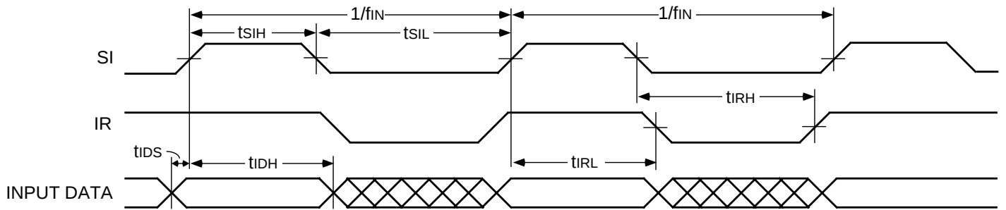
Figure 2. Input Timing
