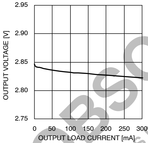
Figure 5. Load Regulation
