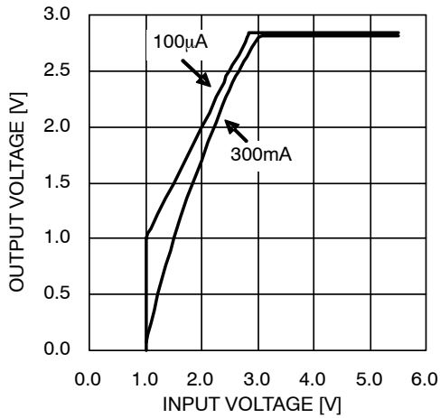
Figure 3. Dropout Characteristics
