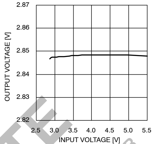
Figure 4. Line Regulation
