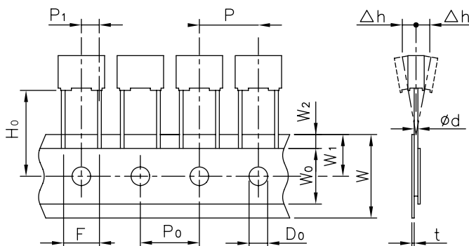
Figure 2 – Lead Space 7.5 mm
