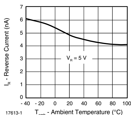
Fig. 8 - Reverse Current vs. Ambient Temperature
