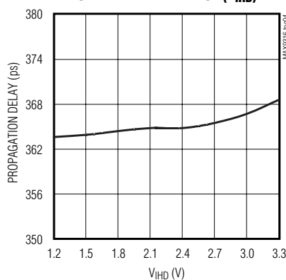
PROPAGATION DELAY vs. HIGH VOLTAGE OF DIFFERENTIAL INPUT ( V_{IHD} )
