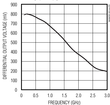
DIFFERENTIAL OUTPUT VOLTAGE ( V_{OH} - V_{OL} ) vs. FREQUENCY
