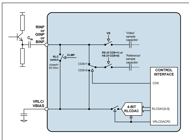
Figure 16 CDS/non-CDS Input Configuration
