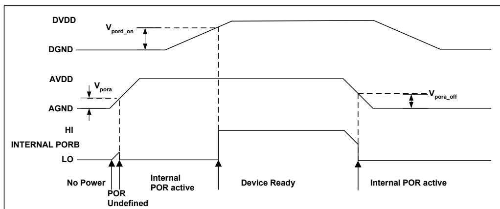
Figure 11 Typical Power up Sequence where AVDD is Powered before DVDD
