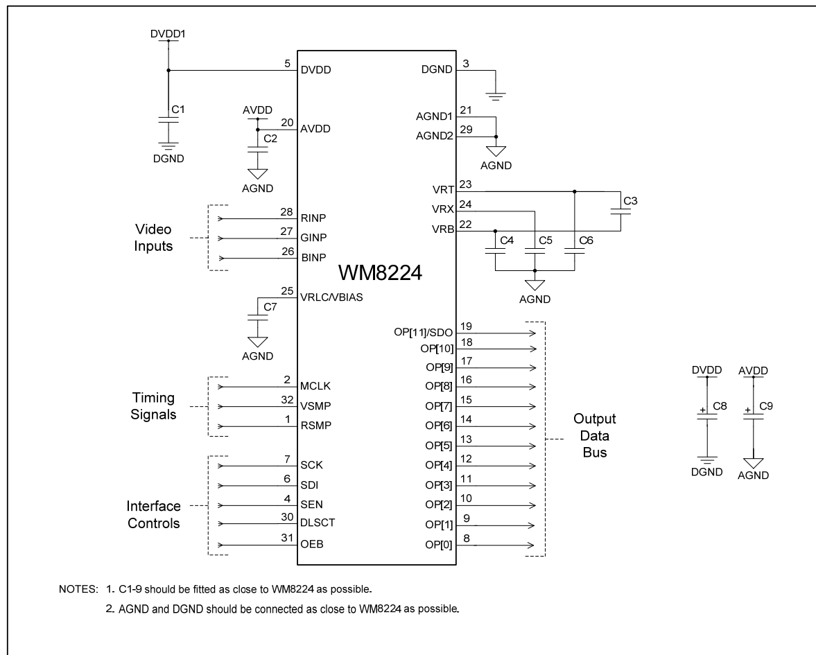
Figure 39 External Components Diagram
