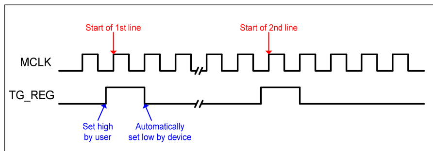
Figure 25 Start of Line Indicator Using TG_REG
