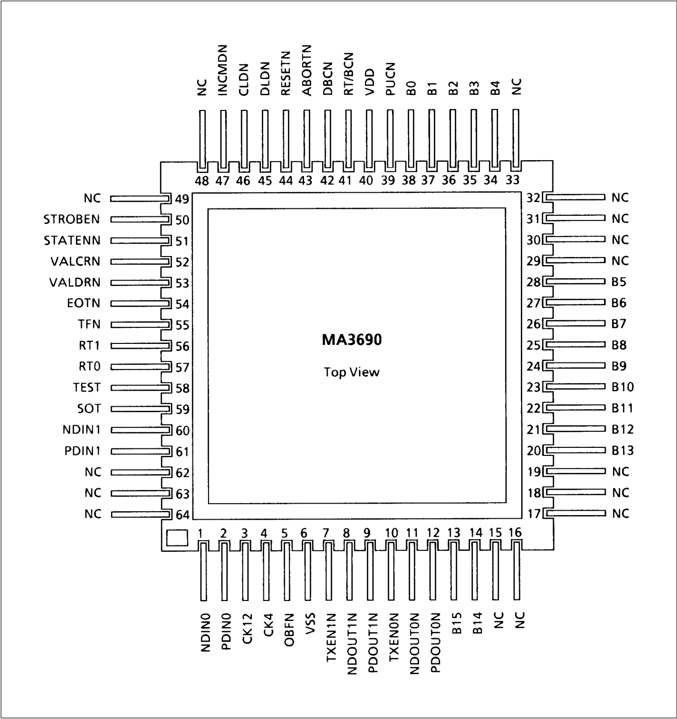
Figure 43b: 64-Lead Topbrazed Flatpack (Package Style F)
