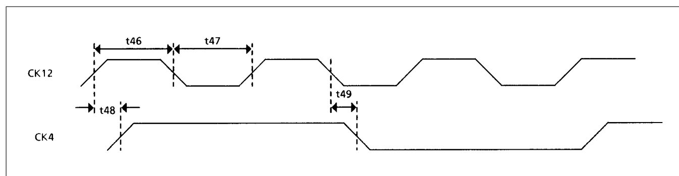
Figure 14: Clock Timing
