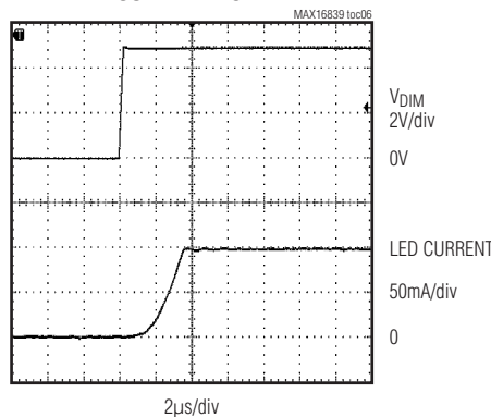
LED CURRENT RISE TIME
