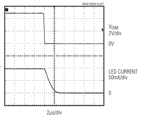
LED CURRENT FALL TIME
