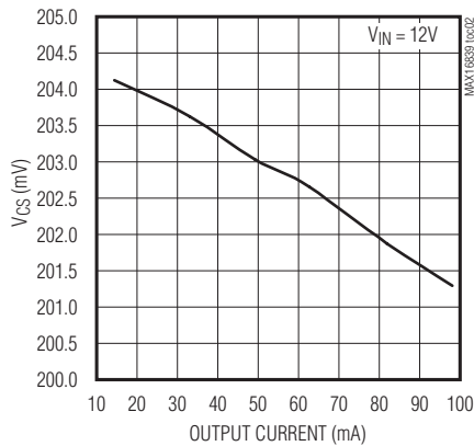
V_{CS} vs. OUTPUT CURRENT
