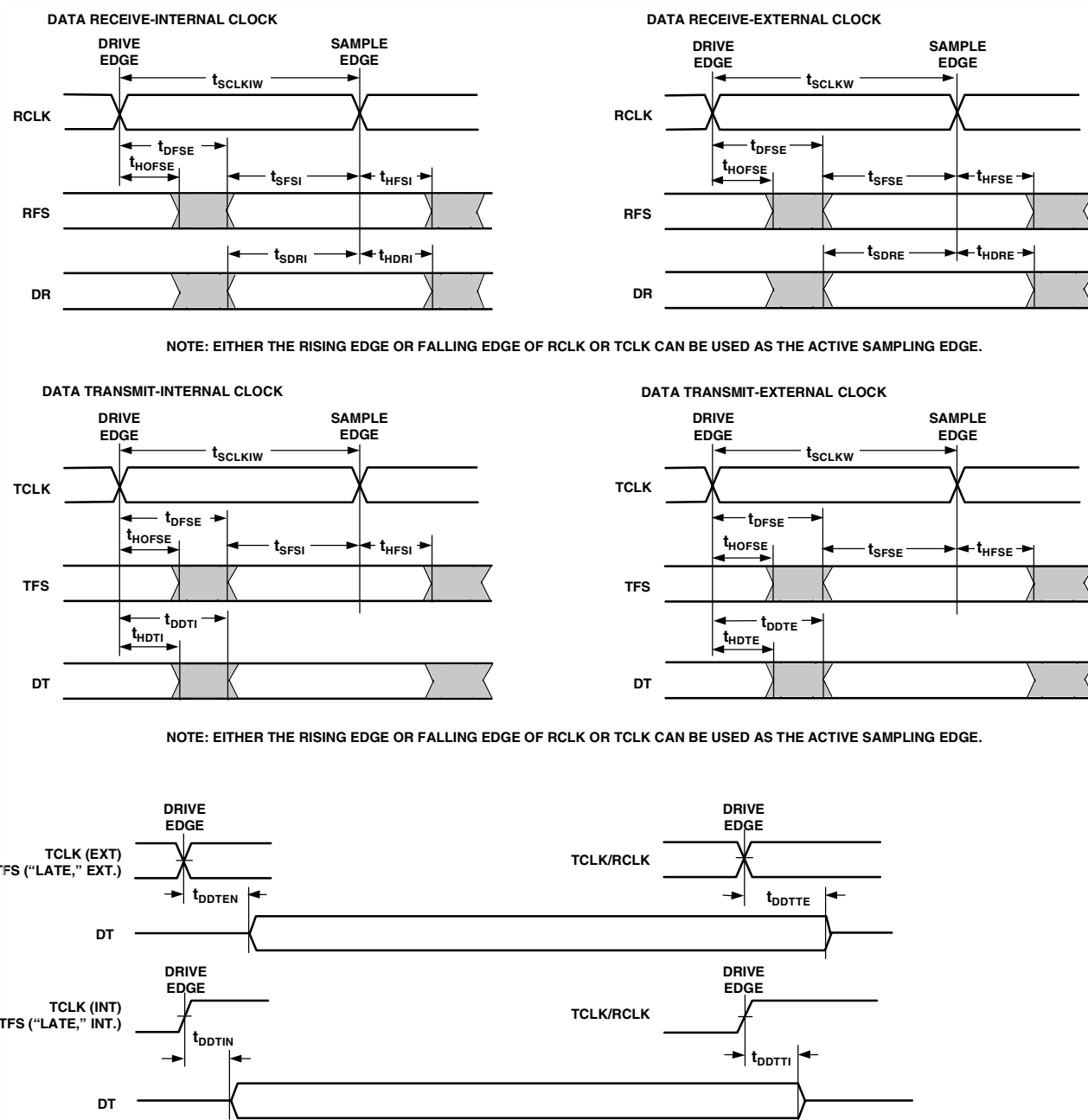
Figure 12. Serial Port
