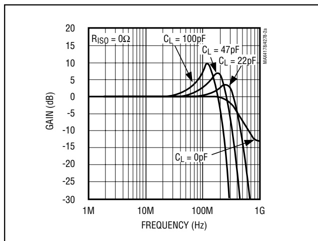
Figure 2a. MAX4178 Small-Signal Gain vs. Frequency with Capacitive Load
