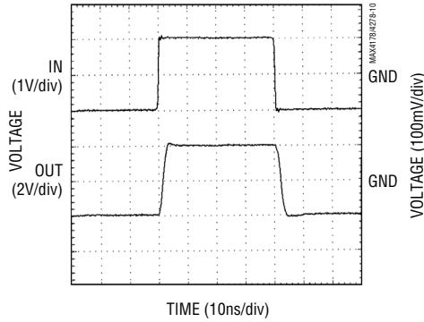
MAX4278 LARGE-SIGNAL PULSE RESPONSE ( C_L = 0pF )
