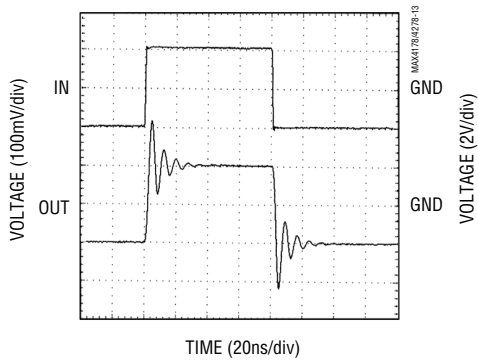
MAX4278 LARGE-SIGNAL PULSE RESPONSE ( C_L = 50pF )
