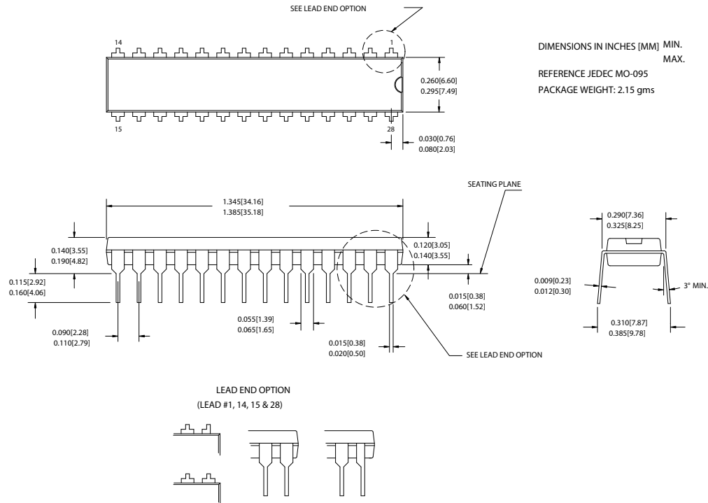
Figure 7. 28-pin (300-Mil) PDIP (51-85014)
