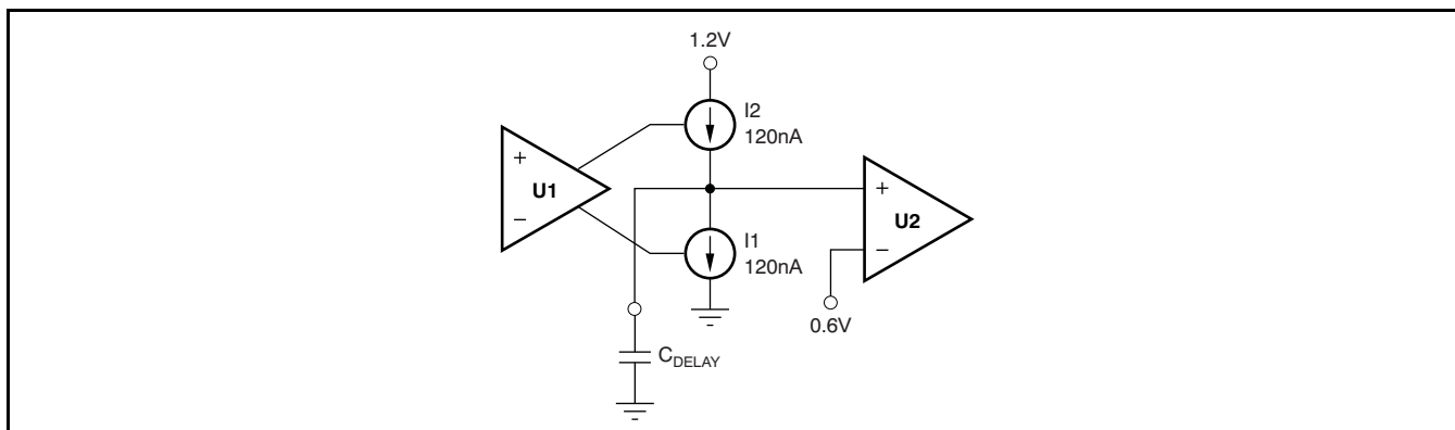
Figure 34. Simplified Model of the Comparator 2 Delay Circuit
