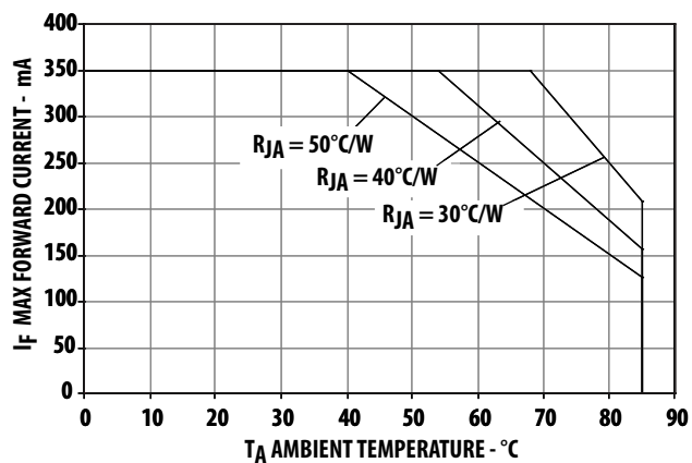
Figure 5. Maximum forward current vs. ambient temperature Derated based on T_{J\text{MAX}} = 110^{\circ}\text{C} , R_{\theta JA} = 30^{\circ}\text{C/W} / 40^{\circ}\text{C/W} and 50^{\circ}\text{C/W}
