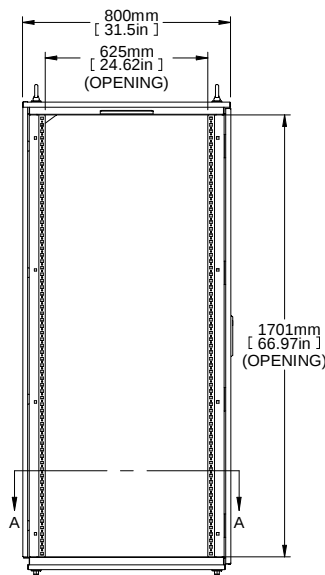
L.S. VIEW
