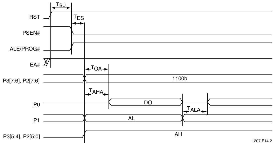
FIGURE 13-23: BYTE-VERIFY
