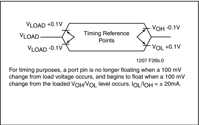
FIGURE 13-9: FLOAT WAVEFORM
