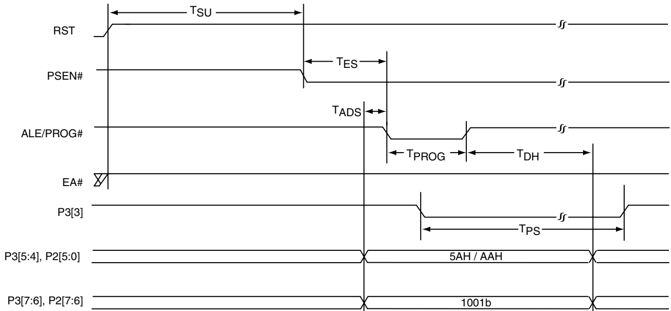
FIGURE 13-22: Prog-SC0 / Prog-SC1
