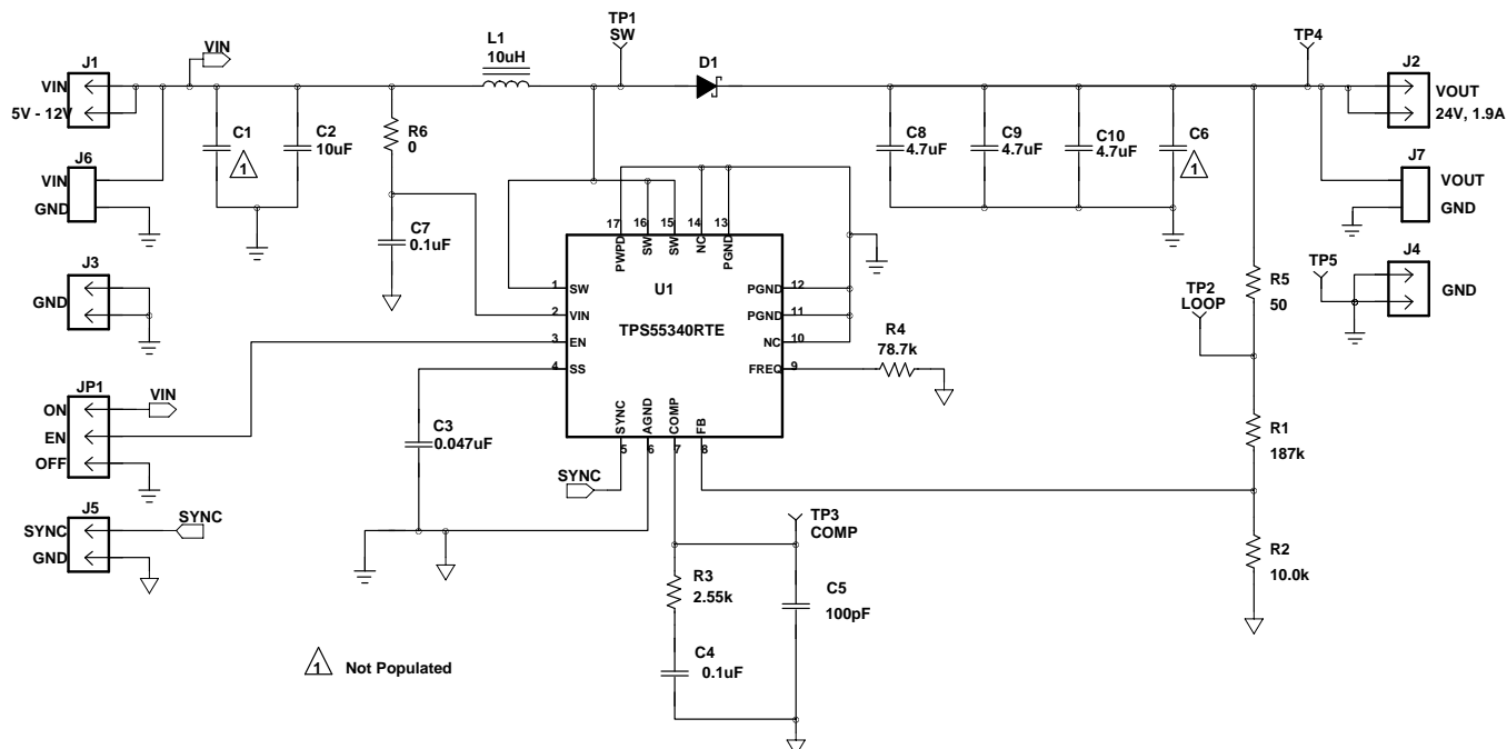
Figure 22. TPS55340EVM-017 Schematic
