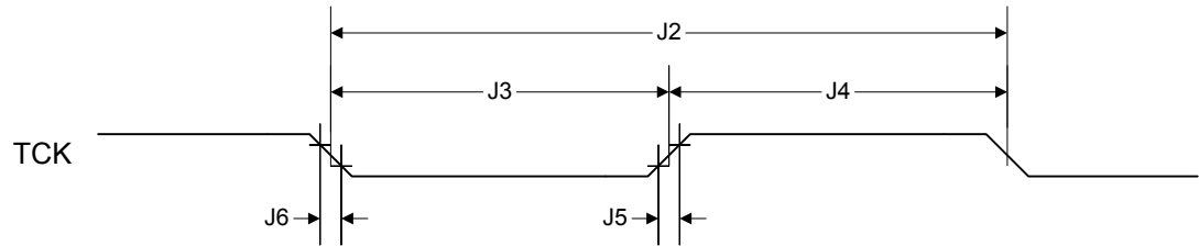
Figure 32-2. JTAG Test Clock Input Timing
