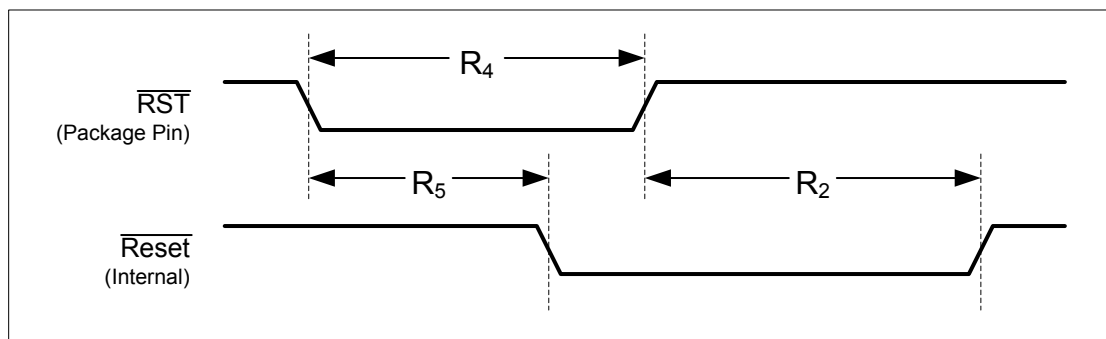
Figure 32-11. External Reset Timing ( \overline{\text{RST}} )
