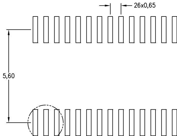
Example Non Soldermask Defined Pad
