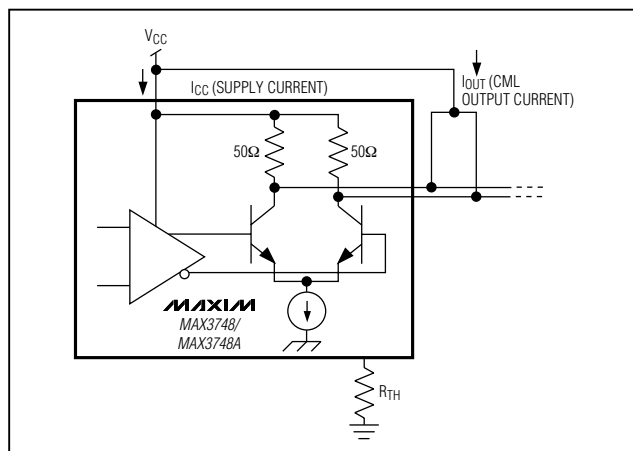
Figure 1. Power-Supply Current Measurement
