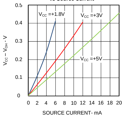
TS9001-1 Output Voltage High vs Source Current
