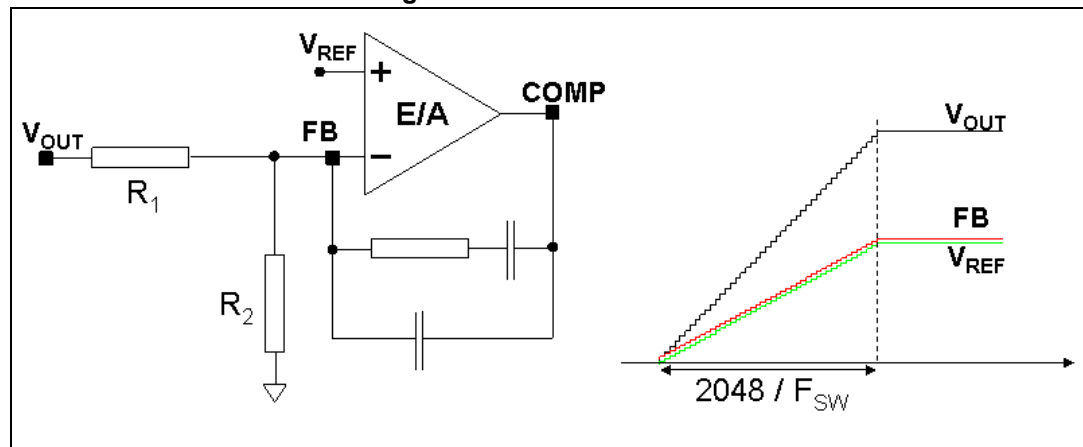
Figure 7. Soft-start scheme
