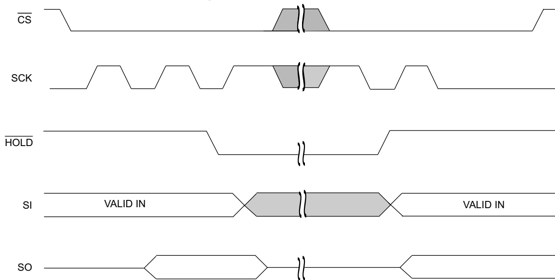
Figure 12. HOLD Operation [2]
