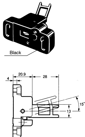
Adjustable Mounting (Horizontal/Vertical) D4DS-K5
