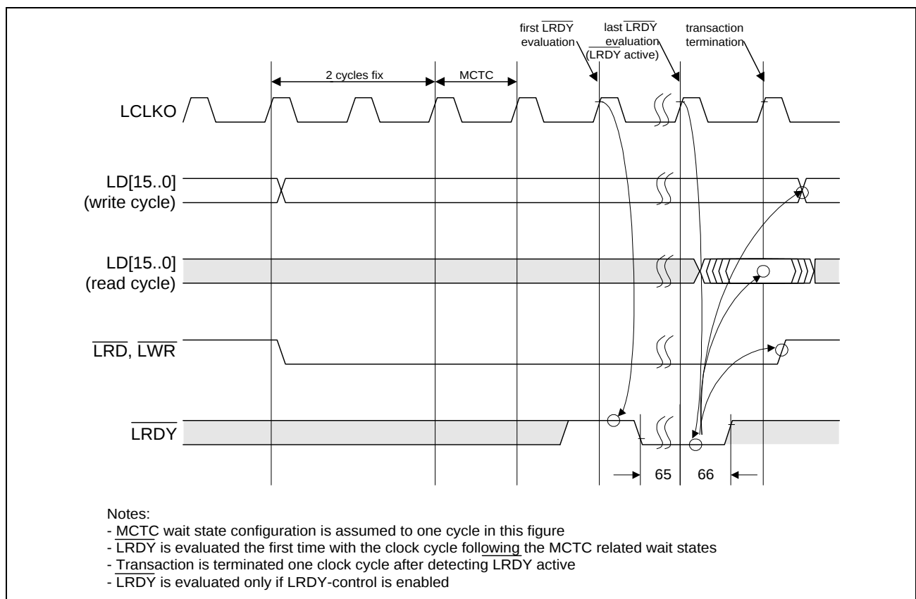
Figure 28 \overline{\text{LRDY}} Timing
