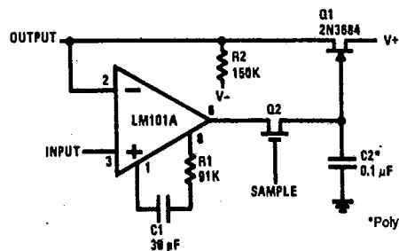
Low Drift Sample and Hold
