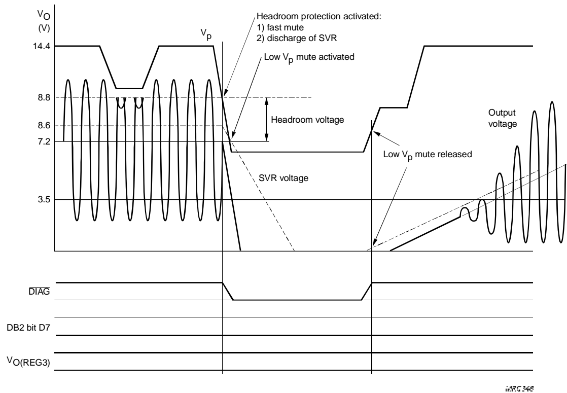
Fig.13 Low V_p behaviour at V_p > 5.5 V.
