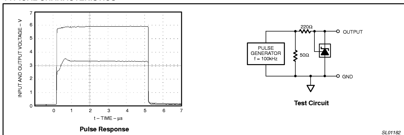
Figure 14. Pulse Response
