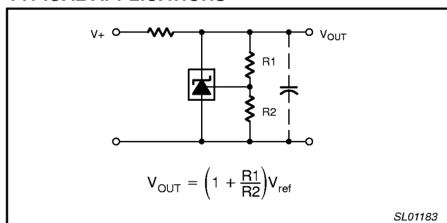
Figure 18. Shunt Regulator
