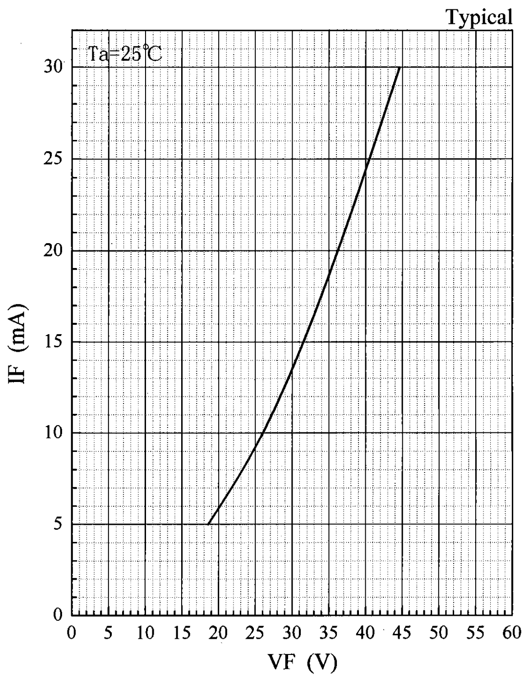
Fig.1 Forward characteristic[VF-IF]
