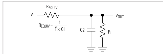
Figure 3b. Equivalent Circuit
