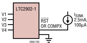
Figure 2. \overline{\text{RST}} , COMPX V_{\text{OL}} Test
