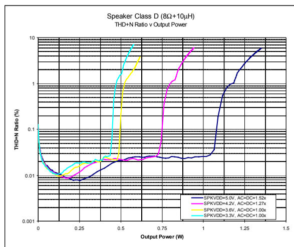
Speaker Class D into 8\Omega + 10\mu\text{H}
