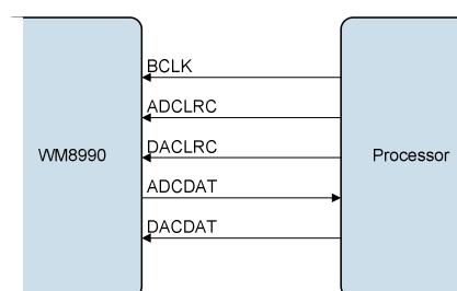
Figure 52 Slave Mode
