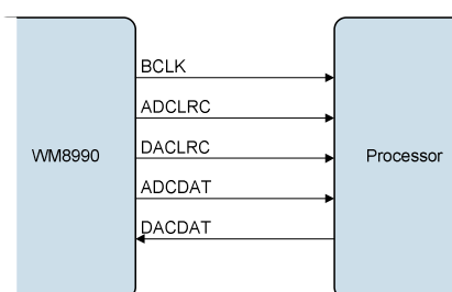
Figure 51 Master Mode
