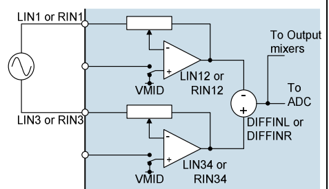
Figure 22 Fully Balanced Differential Input
