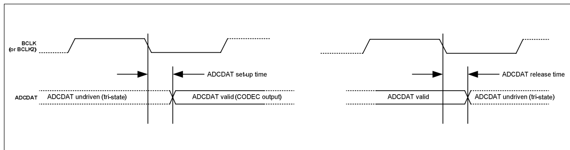
Figure 7 Digital Audio Data Timing - TDM Mode
