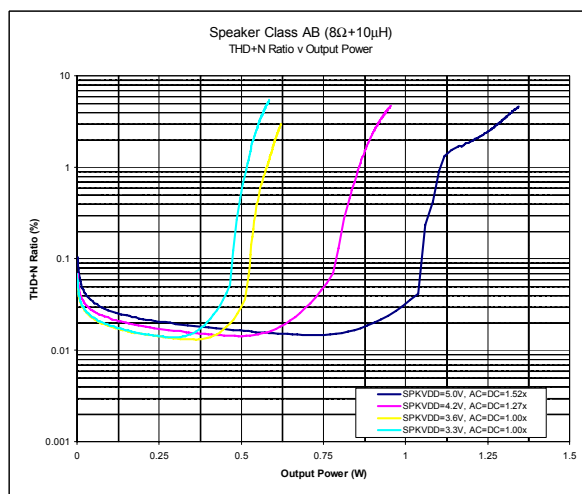
Speaker Class AB into 8\Omega + 10\mu\text{H}
