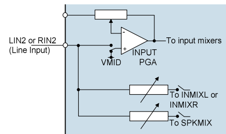
Figure 20 LIN2 or RIN2 as Line Inputs
