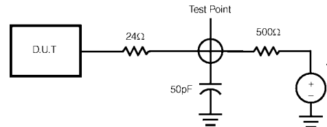
Load for Enable and Disable Times
