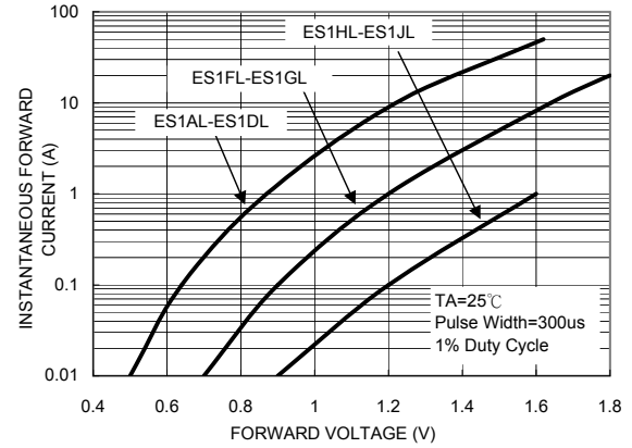
FIG. 2 TYPICAL FORWARD CHARACTERISRICS
