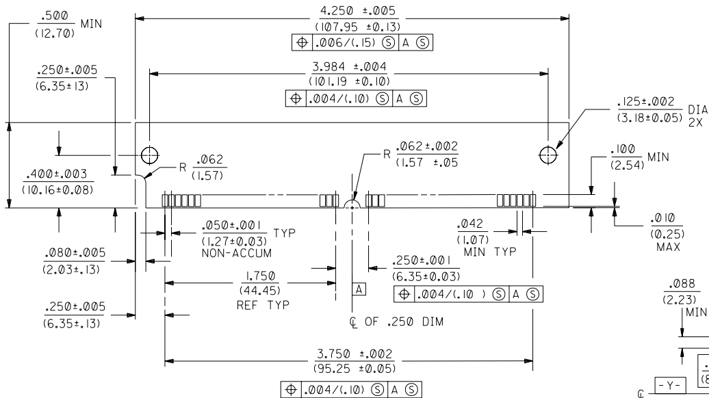
"SIMM" P.C. BOARD LAYOUT
