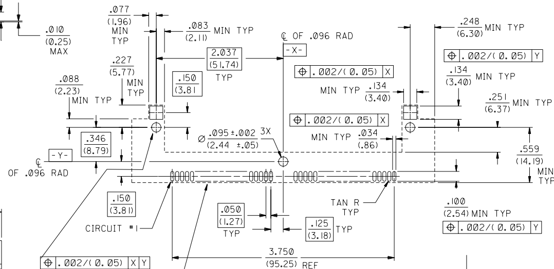
RECOMMENDED SOCKET P.C. BOARD PAD PATTERN
