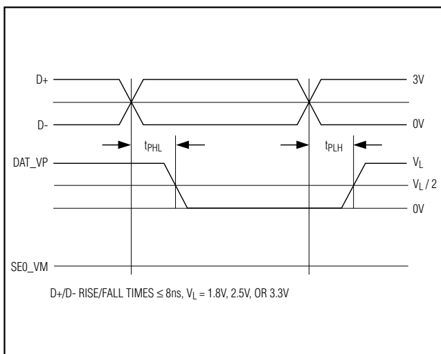
Figure 10. D+/D- to DAT_VP, SE0_VM Propagation Delays (DAT_SE0 Mode)
