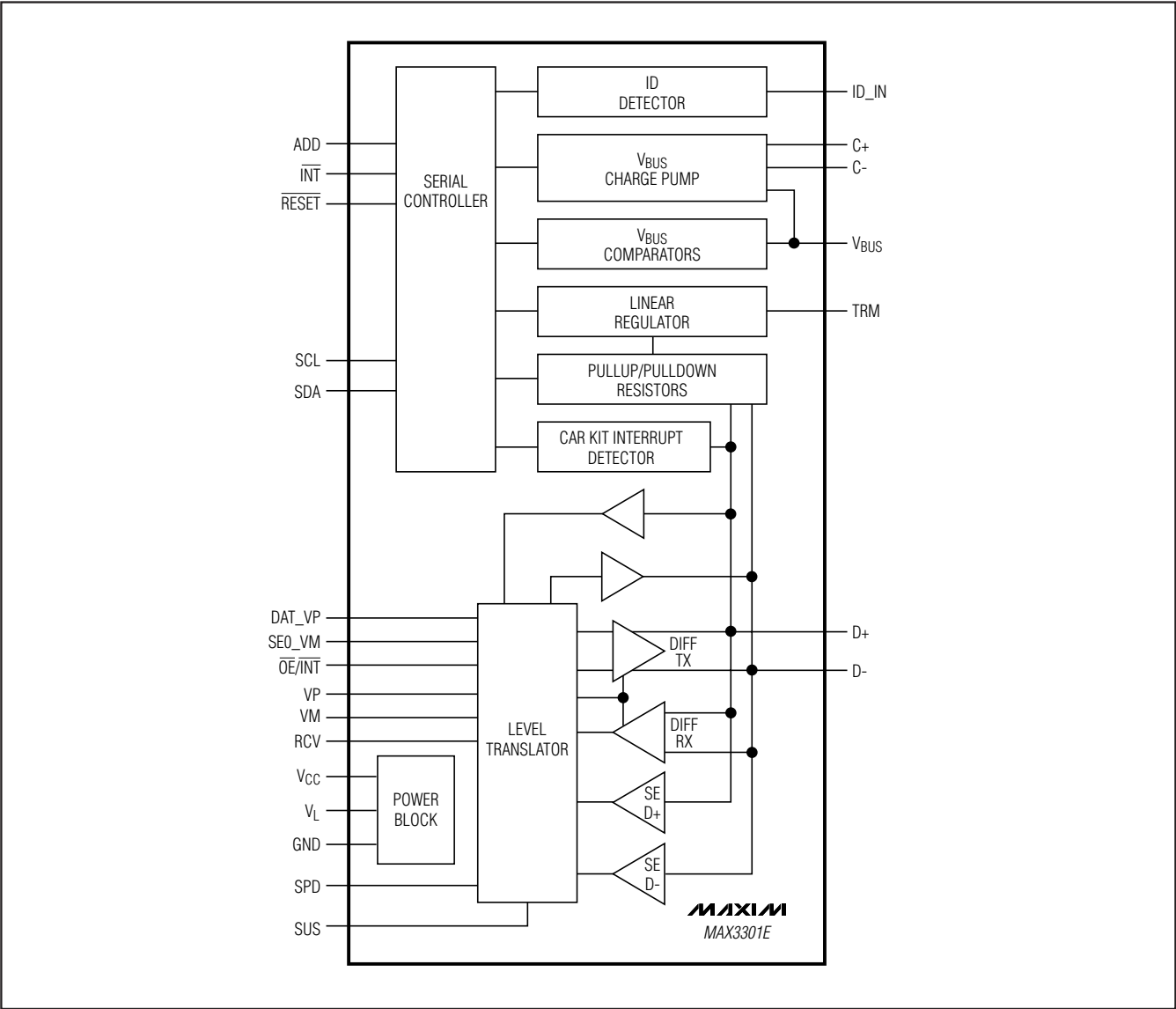
Figure 11. Block Diagram
