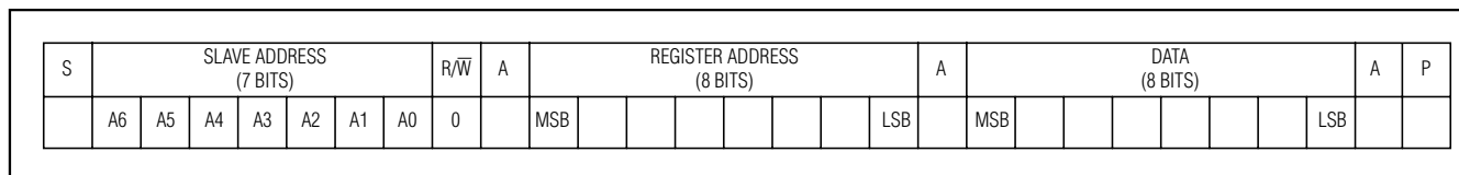
Figure 18. Write-Byte Format
