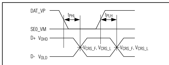
Figure 7. Timing of DAT_VP, SE0_VM to D+/D- in DAT_SE0 Mode (dat_se0 = 1)
