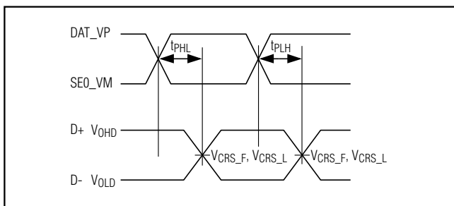
Figure 6. Timing of DAT_VP, SE0_VM to D+, D- in VP_VM Mode (dat_se0 = 0)
