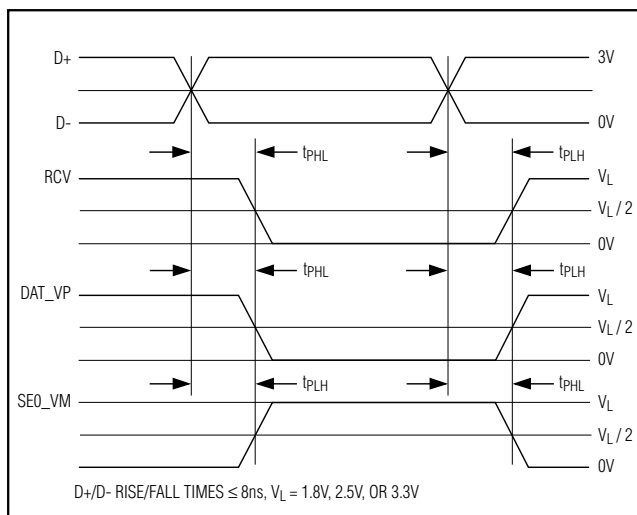
Figure 9. D+/D- to RCV, DAT_VP, SE0_VM Propagation Delays (VP_VM Mode)
