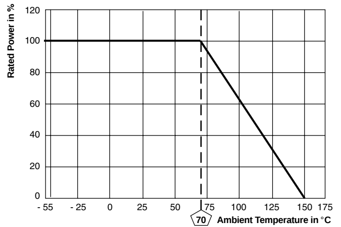
Derating
