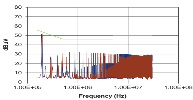
NXJ2S2415MC (Average)
