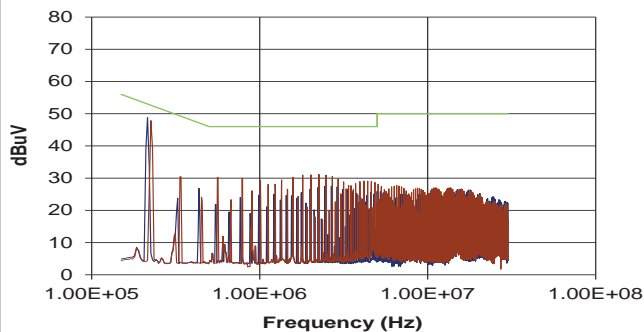
NXJ2S2405MC (Average)
