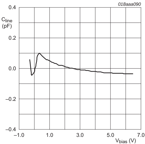
Deviation from typical capacitance normalized at V_{bias} = 2.5 V
