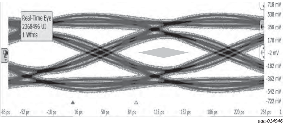
148.5 MHz test frequency Measured at TP2 with worst cable emulator, reference cable equalizer and worst case negative skew, device powered.
