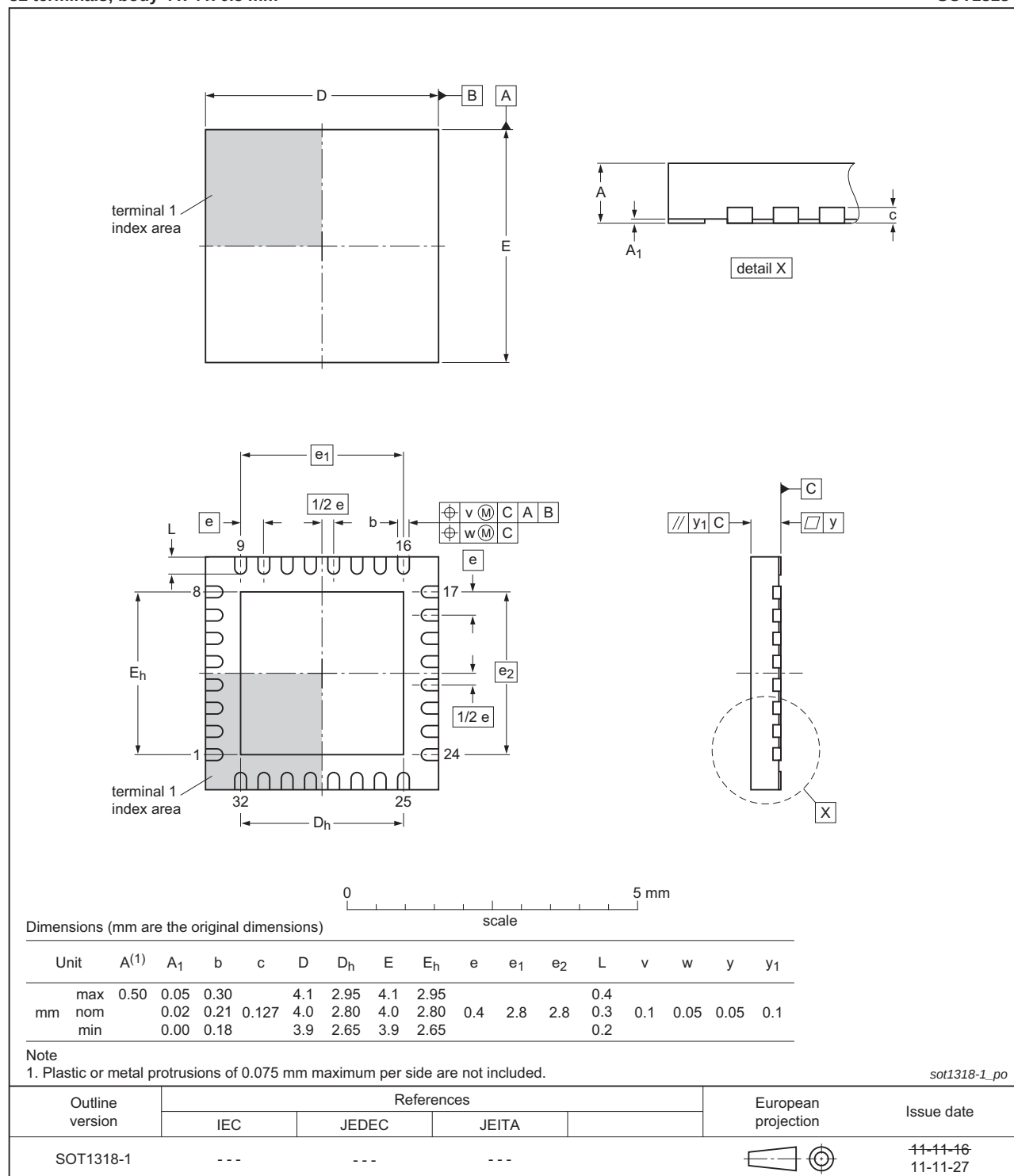
Fig 30. Package outline SOT1318-1 (HXQFN32)
